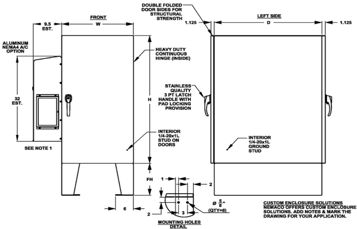
FIG. 1 - NEMA 4 - "PCE" Aluminum 19" RACK SERVER ENCLOSURE - EXTERIOR DIMENSIONS
