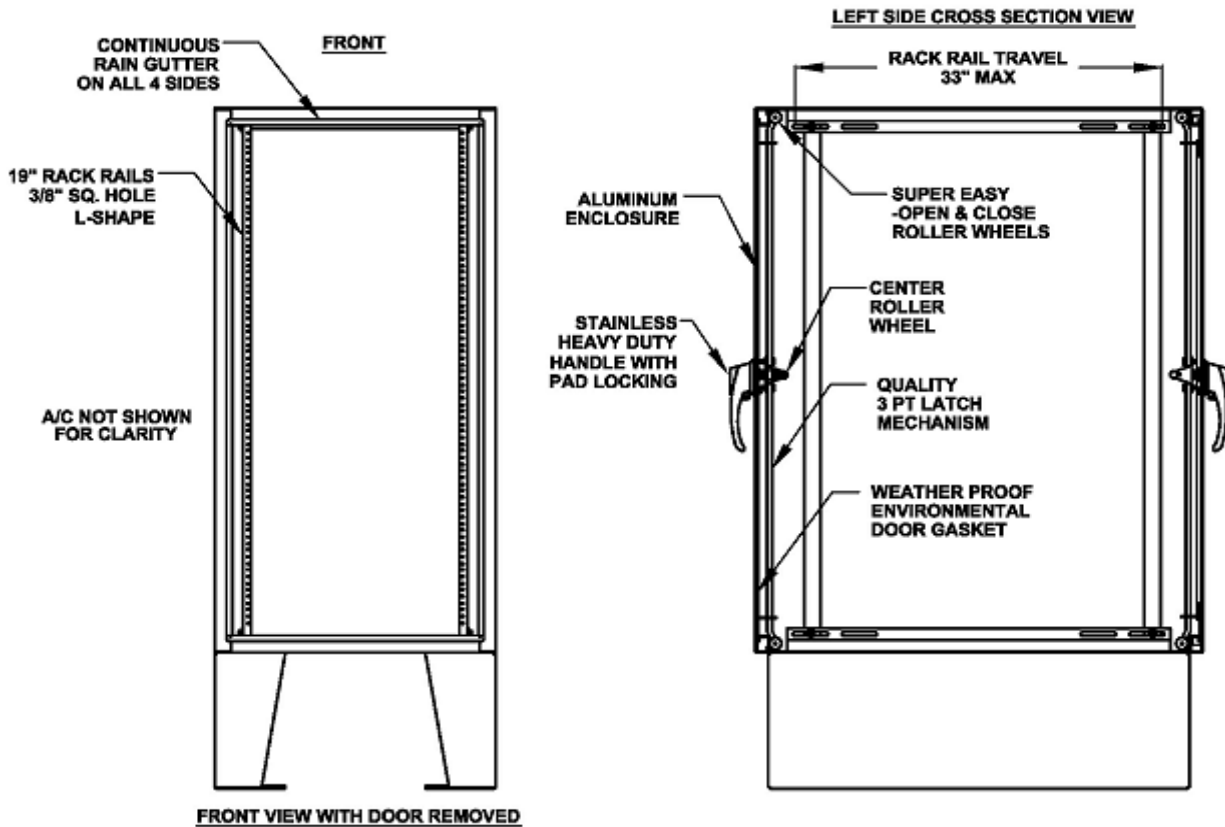
FIG. 2 - NEMA 4 - "PCE" Aluminum 19" RACK SERVER ENCLOSURE - CABINET FEATURES
